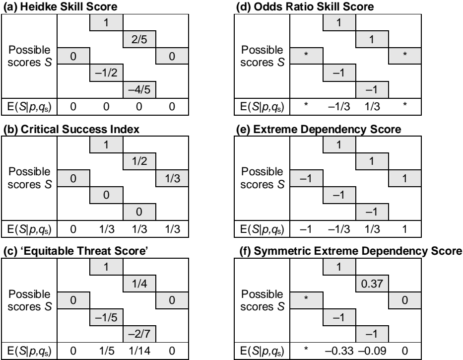
Figure 4. Values of the scores for each of the contingency tables given in Fig. 3, together with the expected score for each value of sample forecast rate of occurrence at the bottom of each column, E(S|p, q_s) . Measures are only truly equitable if they have E(S|p, q_s) = 0 in each column. Note that unlike in panel a of Fig. 2, panel a of this figure corresponds only to the Heidke Skill Score and not the Peirce Skill Score, which is different in the case of q_s = 2/3 . The asterisks in panels d and f indicate that a value is undefined.
