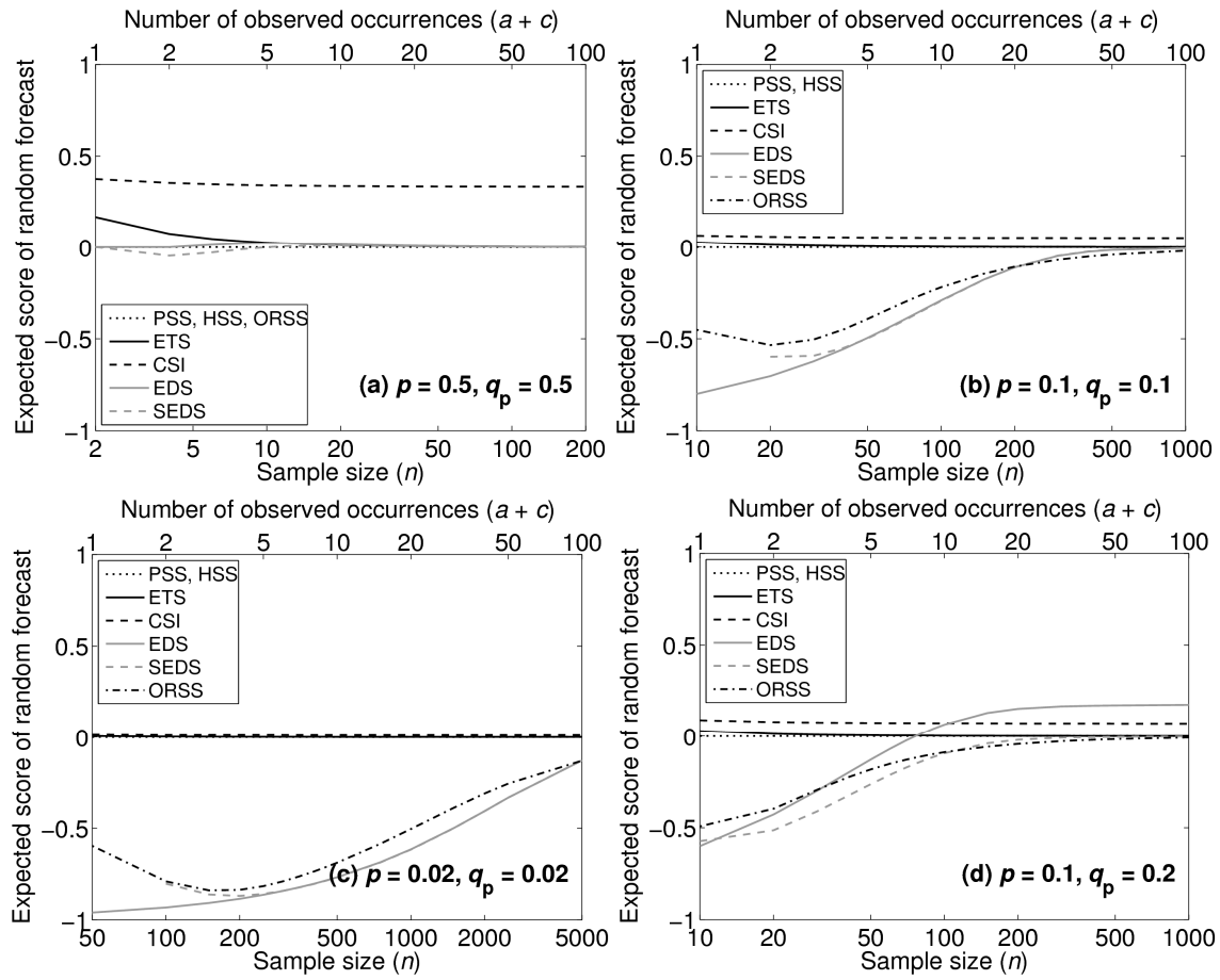
Figure 5. The expected values of a number of verification measures, E(S|p) , versus sample size, for random forecasting systems with base rate p and population forecast probability of occurrence q_p of (a) p = q_p = 0.5 , (b) p = q_p = 0.1 , (c) p = q_p = 0.02 , and (d) p = 0.1 and q_p = 0.2 . The undefined values are removed from consideration when calculating SEDS, but when these occupy more than 25% of probability space, SEDS is not plotted; this only affects panels b and c.
