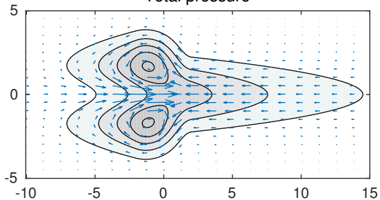
Total pressure
