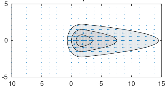
Kelvin pressure
