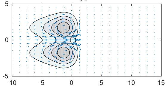
Rossby pressure
