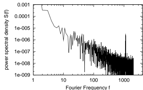
FIG. 13: FFT of the beat frequency for two oscillators close to phase locking.
