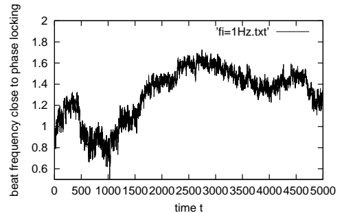
FIG. 12: Beat frequency between two radio frequency oscillators close to phase locking.
