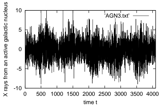
FIG. 9: X ray variability from an active galactic nucleus (AGN).
