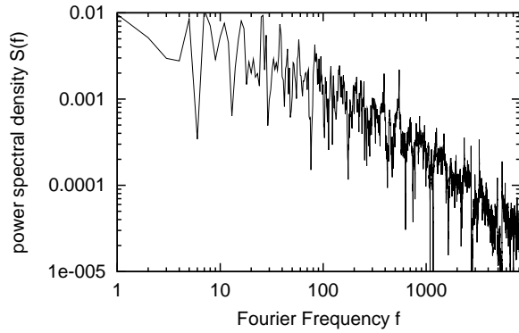
FIG. 5: Power spectral density (FFT) of the error term of Mangoldt function \Lambda(n) .
