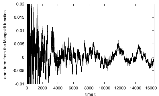
FIG. 4: Error term in the Mangoldt function \Lambda(n) .
