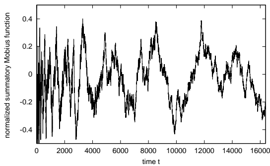
FIG. 1: The normalized summatory Möbius function M(t)/t^{1/2}
