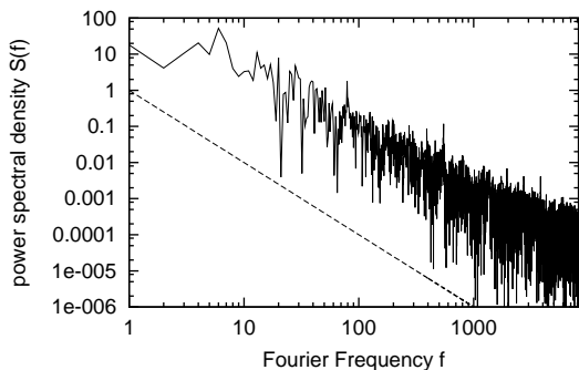
FIG. 2: The power spectral density (FFT) of the normalized summatory Möbius function M(t)/t^{1/2} in comparison to the power law 1/f^2 (dotted line).
