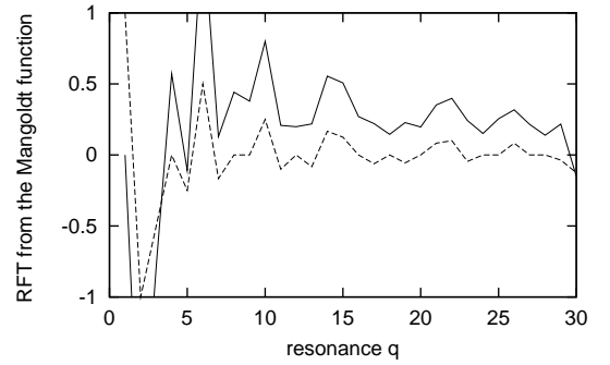
FIG. 8: Ramanujan-Fourier transform (RFT) of the error term (upper curve) of new Mangoldt function b(n) in comparison to the function \mu(q)/\phi(q) (lower curve).
