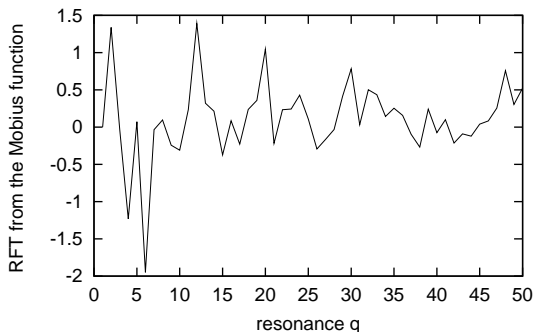
FIG. 3: The Ramanujan-Fourier transform (RFT) of the normalized summatory Möbius function shown in Fig.1.
