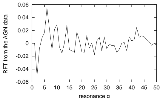
FIG. 11: Ramanujan-Fourier transform (RFT) of X ray variability of an AGN.
