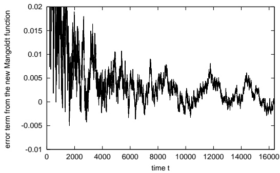
FIG. 6: Error term in the new Mangoldt function b(n) .
