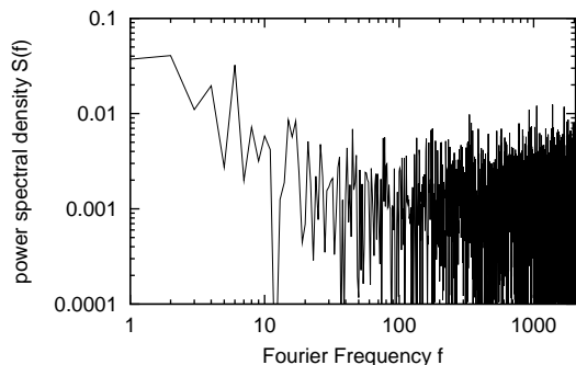
FIG. 10: Power spectral density (FFT) of X ray variability from an AGN.
