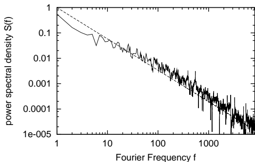
FIG. 7: Power spectral density (FFT) of the error term in new Mangoldt function b(n) in comparison to the power law 1/f^{2\alpha} , with \alpha = (\sqrt{5} - 1)/2 the golden mean.
