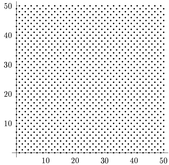
FIGURE 2. Odd Gaussian integers.
