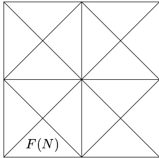
FIGURE 6. Reflection symmetries modulo N .
