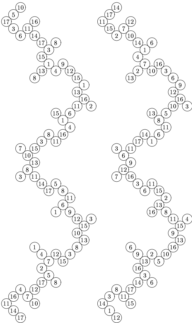
FIGURE 11. Left: Component of size 71 modulo 4 + i . Right: Component of size 71 modulo 4 - i .
