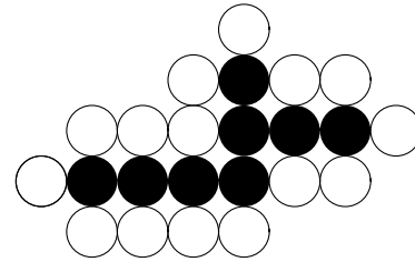
FIGURE 4. A connected set of black Go stones captured by white.
