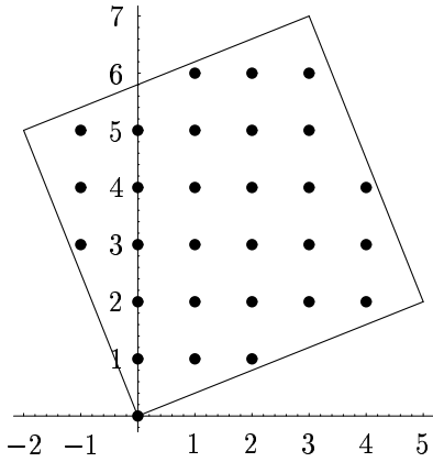
FIGURE 3. Fundamental domain for 5 + 2i of norm 29.
