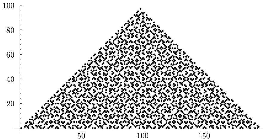
FIGURE 9. Walks relatively prime to 2 \cdot 3 \cdot 5 \cdot 13 .
