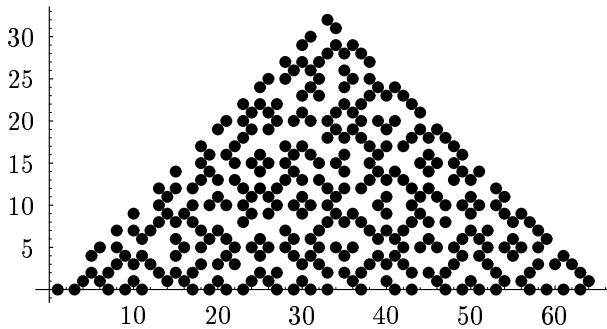
FIGURE 7. There is no unbounded walk prime to 2 \cdot 5 \cdot 13 of step size \sqrt{2} .
