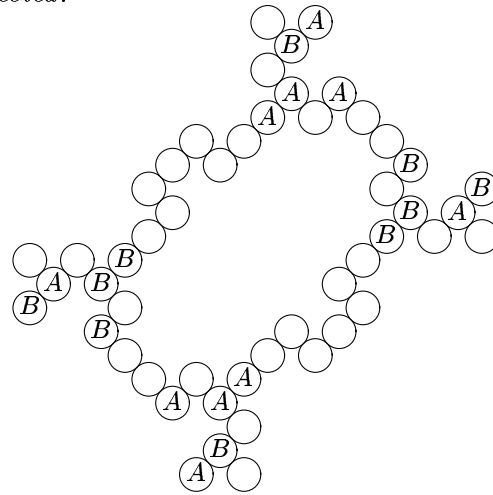
FIGURE 8. The largest admissible connected components.
