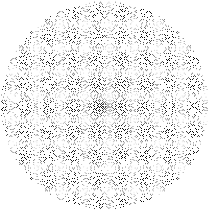
FIGURE 1. Gaussian primes at distance at most 100 from the origin.
