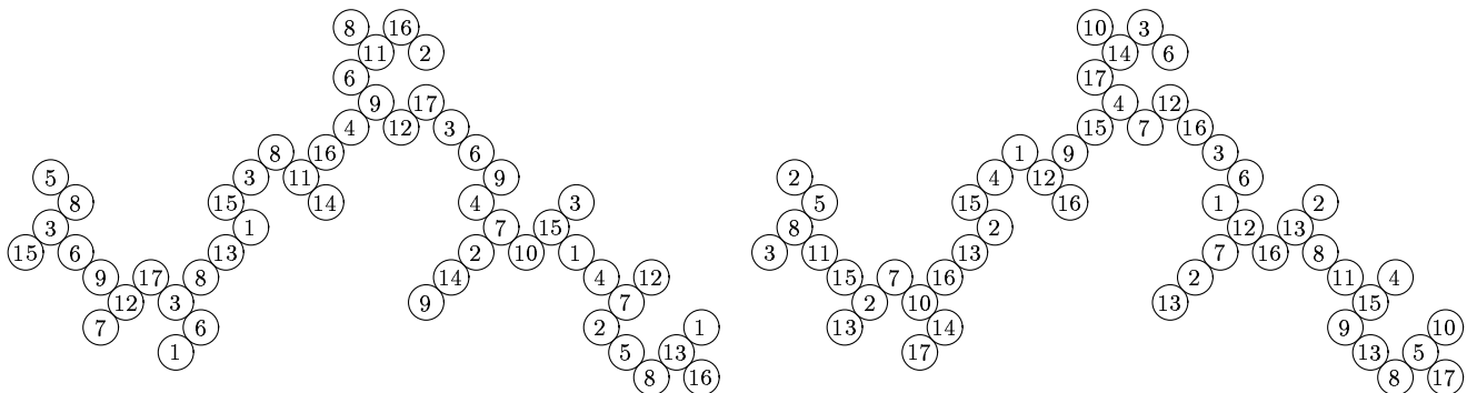
FIGURE 10. Left: Component of size 51 modulo 4 + i . Right: Component of size 51 modulo 4 - i .
