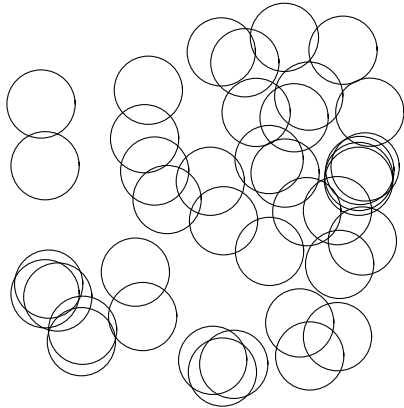
FIGURE 5. Poisson blob model of intensity \lambda = 0.4 .
