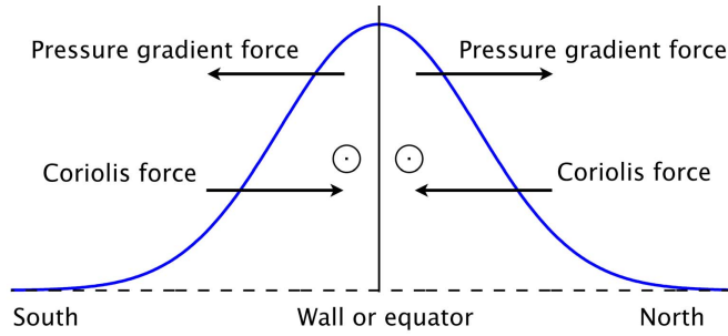
Fig. 8.4 Balance of forces across a Kelvin wave; the solid line is the fluid surface and the phase speed is directed out of the page. Beneath a crest, as shown, the fluid flow is in the direction of the phase speed and produces Coriolis forces in the directions shown, so balancing the pressure gradient forces. If the wave were travelling in the other direction no such geostrophic balance could be achieved.
