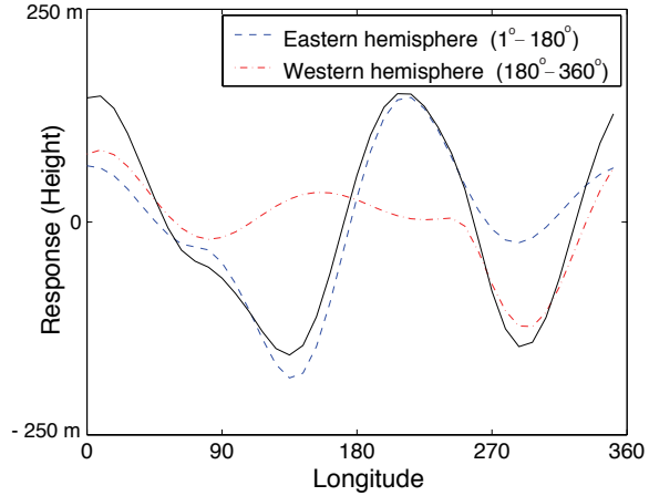
Fig. 16.12 The solution of the upper left-hand panel Fig. 16.11 (solid line), and the solution divided into two contributions (dashed lines), one due to the topography only of the western hemisphere (i.e., with the topography in the east set to zero) and the other due to the topography only of the eastern hemisphere.
