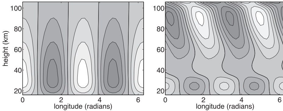
Fig. 17.28 Snapshots of the wave streamfunction in the steady case (forcing of 200) in the left panel and in the oscillatory case (forcing of 300) in the right panel. Zero contour is heavy.
