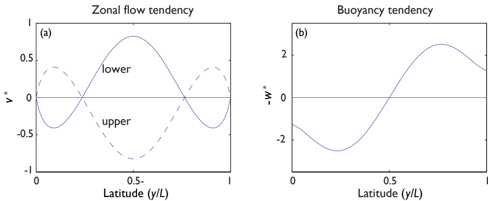
Fig. 10.5 (a) The tendency of the zonal mean flow ( \partial \bar{u}/\partial t ) just below the upper lid (dashed) and just above the surface (solid) in the Eady problem. The vertically integrated tendency is zero. (b) The vertically averaged buoyancy tendency.
