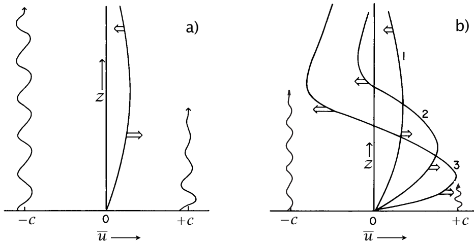
Fig. 17.17 Schema of the initial instability leading to the QBO. 30 The solid lines show the zonal flow, the wavy arrows indicate the gravity-wave penetration from below and the double arrows indicate wave-induced acceleration. Initially, as in the left panel, a small eastward perturbation is added to a stationary mean flow. The eastward moving wave is preferentially absorbed and the perturbation is amplified and then descends, with the right panel showing the zonal flow at the successive times indicated, with the gravity wave penetration illustrated at t = 3 . After the flow develops an eastward component the westward wave penetrates higher before being absorbed, inducing a westward flow aloft that then itself descends, making the eastward anomaly thinner. Subsequent stages and the development of a periodic oscillation are illustrated in Fig. 17.18.
