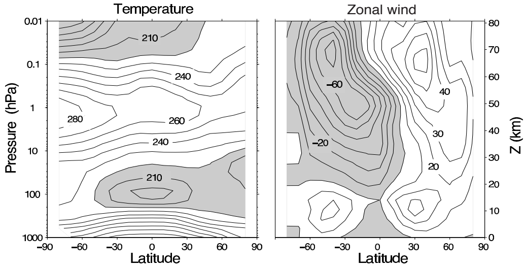
Fig. 17.2 The zonally averaged temperature and zonal wind in January. The temperature contour interval is 10 K, and values less than 220 K are shaded. Zonal wind contours are 10 \text{ m s}^{-1} and negative (westward) values are shaded. 5
