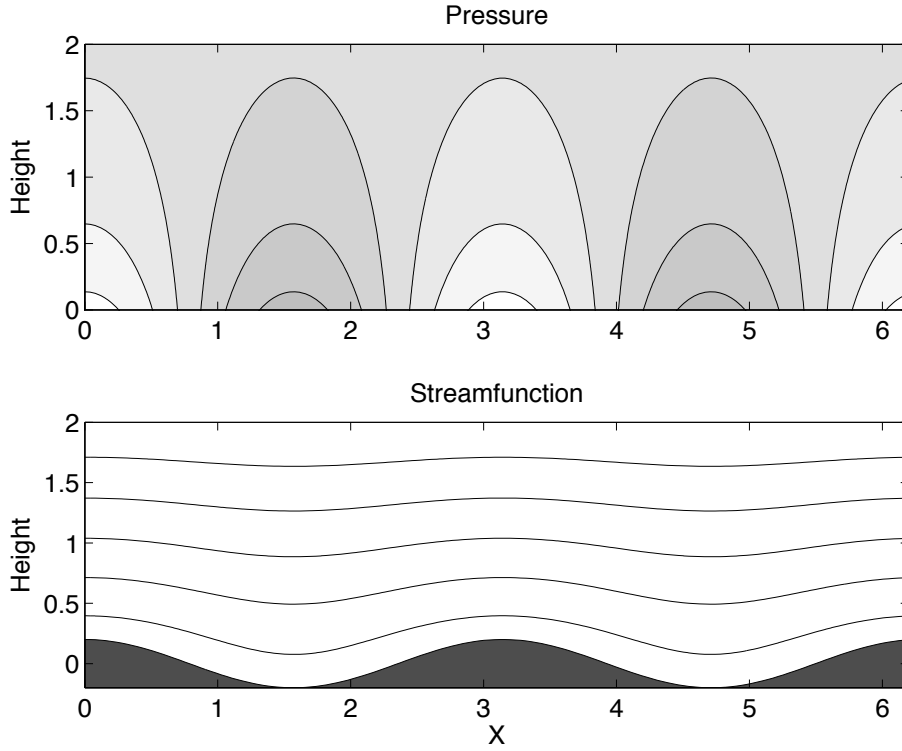
Fig. 7.18 Solutions for the flow over a sinusoidal ridge, using (7.190), in the short wave limit and with m = i . The top panel shows phase lines of pressure, with darker gray indicating higher pressure. The bottom panel shows contours of the total streamfunction, \psi - Uz , with flow coming in from the left, and the topography itself (solid). The perturbation amplitude decreases exponentially with height.
