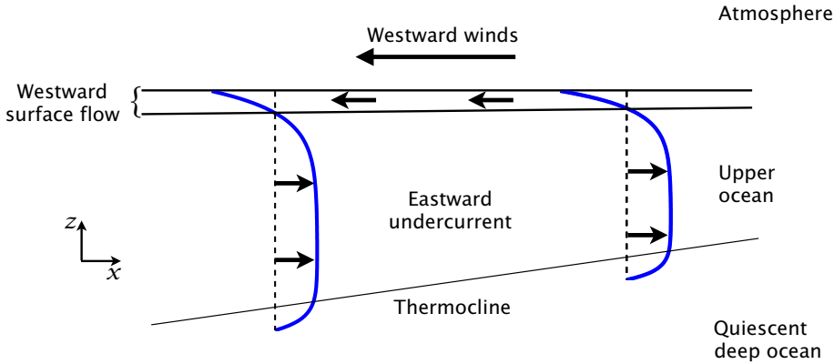
Fig. 22.8 A schematic zonal section of the local model of the undercurrent and thermocline.
