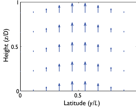
Fig. 10.2 The Eliassen–Palm vector in the Eady problem.
