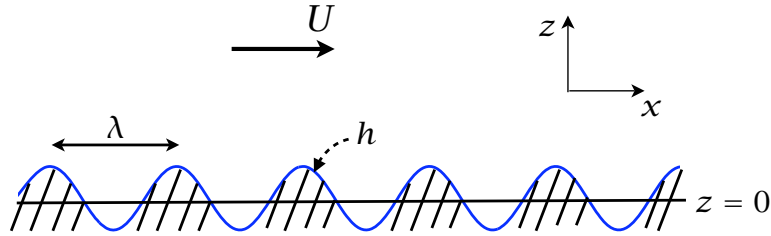
Fig. 7.17 Uniform flow, U , in the x -direction flowing over sinusoidal topography, h . The vertical co-ordinate is stretched, and in reality |h| \ll \lambda .
