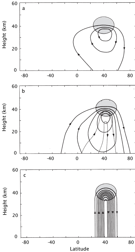
Fig. 17.13 The numerically-computed response of the meridional overturning circulation to a longitudinally symmetric westward force, with the frequency of the forcing decreasing from top to bottom. 19 Contours are streamlines of the residual circulation, with the same uniform interval in all panels, and the shading denotes the forcing region.
