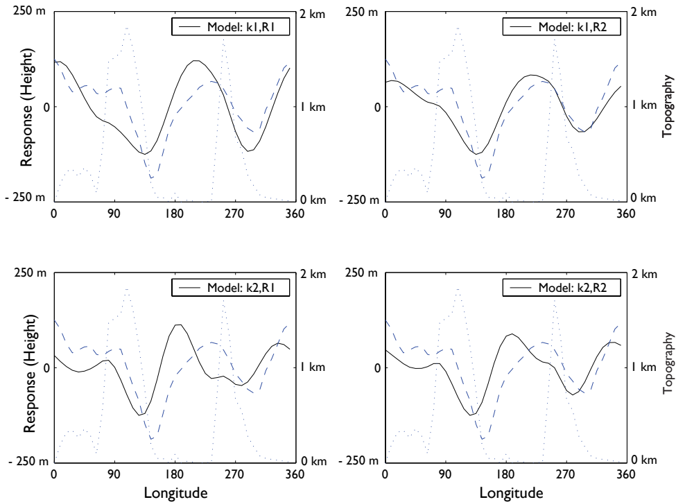
Fig. 16.11 Solutions of the Charney–Eliassen model. The solid lines are the steady solution of (16.86) using the Earth’s topography at 45° N with two values of friction ( R1 \approx 6 days, R2 \approx 3 days) and two values of resonant zonal wavenumber (2.5 for k1 , 3.5 for k2 ), corresponding to zonal winds of approximately 17 and 13 \text{m s}^{-1} . The solutions are given in terms of height, \eta' , where \eta' = f_0 \psi' / g , with the scale on the left of each panel. The dashed line in each panel is the observed average height field at 500 mb at 45° N in January. The dotted line is the topography used in the calculations, with the scale on the right of each panel.
