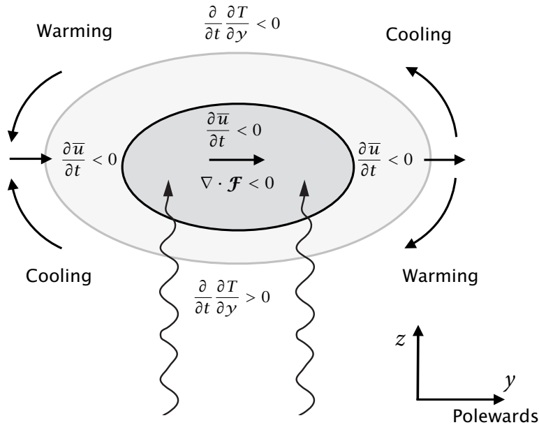
Fig. 17.25 The circulation induced by a patch of negative EP flux divergence ( \nabla \cdot \mathcal{F} < 0 , dark shading). The westward acceleration ( \partial \bar{u} / \partial t < 0 ) occurs there, spreading out over a broader region (light shading). Assuming there is no acceleration far away from the wavebreaking, the temperature response can be inferred from thermal wind, with a warming at the lower poleward end of the breaking, as indicated, and an induced residual circulation as shown by the arrows.
