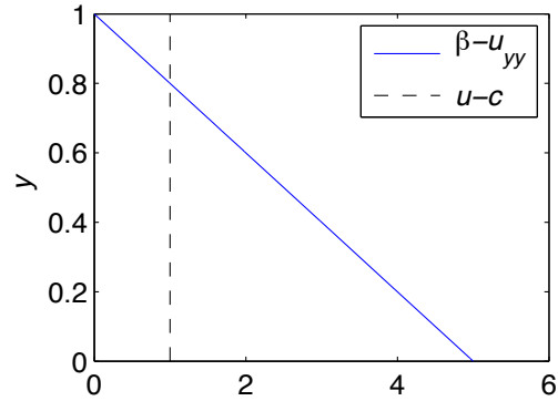
Fig. 16.1 Parameters for the first example considered in section 16.2.2, with all variables nondimensional. The zonal flow is uniform with u = 1 and c = 0 (so that \bar{u}_{yy} = 0 ) and \beta diminishes linearly as y increases polewards as shown. With zonal wavenumber k = 1 there is a turning latitude at y = 0.8 , and the wave properties are illustrated in Fig. 16.2.
