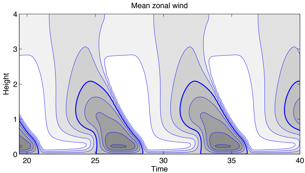
Fig. 17.22 Time height section of nondimensional zonal wind in a numerical solution using (17.70), showing the last 20 time units of the same integration as Fig. ???. Contours are plotted every 0.2 units, positive winds are shaded darker and the zero contour is thicker.
