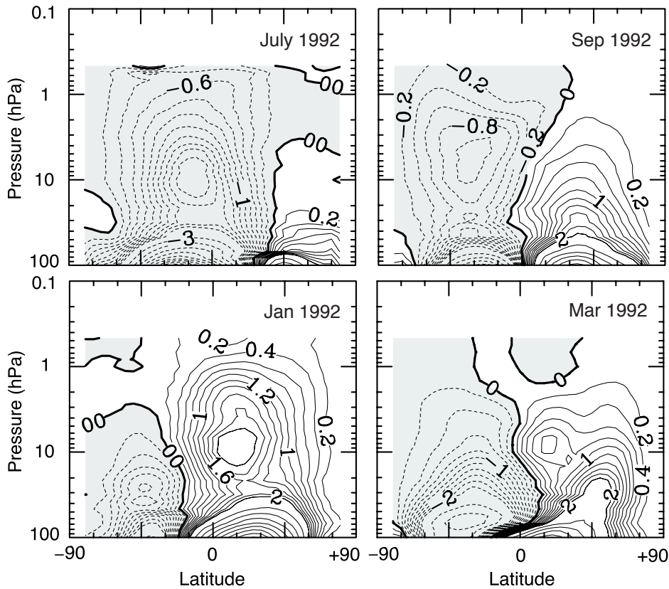
Fig. 17.7 The observed thickness-weighted (residual) streamfunction in the stratosphere, in Sverdrups ( 10^9 \text{ kg s}^{-1} ). The circulation is clockwise where the contours are solid. Note the stronger circulation in the winter hemispheres, whereas the equinoctial circulations (September, March) are more inter-hemispherically symmetric. 13
