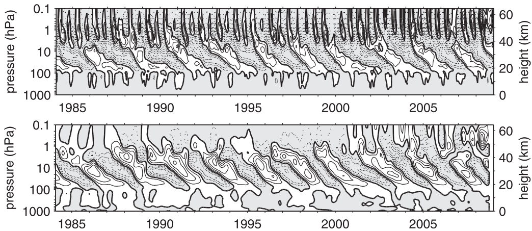
Fig. 17.14 Time height sections of the observed monthly mean equatorial zonal wind for 1984–2010, with the seasonal cycle removed. Contour interval is 5 \text{ m s}^{-1} and grey shading (with dotted contours) denote negative, or westward, winds. In the bottom panel the data are band-passed to retain periods between 9 months and 4 years only. An oscillation, the ‘quasi-biennial oscillation’ or QBO, is quite visible between 20 and 40 km, or about 60 and 3 hPa. 23
