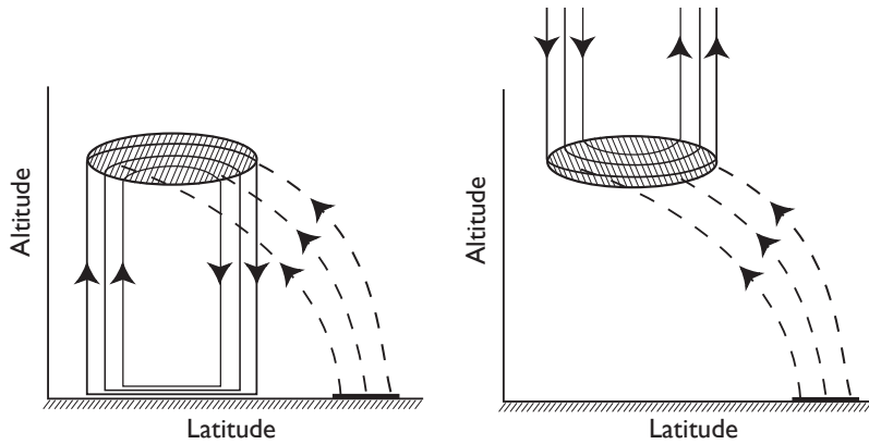
Fig. 17.12 Idealized example of downward control. Left panel: wave activity propagates upwards (dashed lines) from a tropospheric source, breaking and depositing zonal momentum in the shaded region. This induces an overturning circulation (solid lines) below the region of momentum deposition, connecting the region of wave breaking with a frictional boundary layer. Right panel: putative ‘upward control’, which would require a frictional sink above the wave breaking region for the response to be steady.
