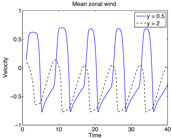
Fig. 17.21 The evolution of the mean zonal wind at two different levels in a numerical solution using (17.70). All the variables are nondimensional, with the only parameter in the problem being viscosity. A small perturbation is added to \bar{u} , and relatively quickly the solution becomes periodic.
