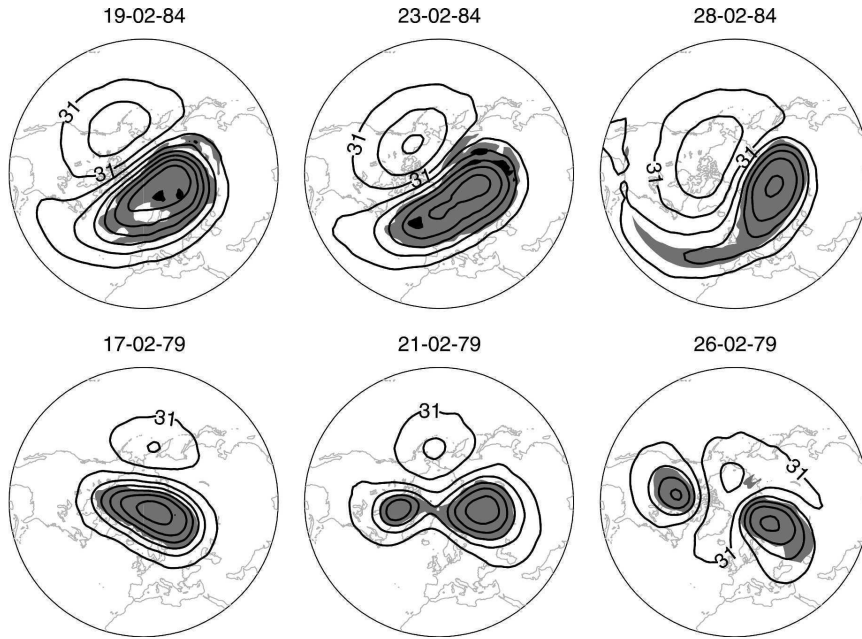
Fig. 17.23 Time sequence of two stratospheric warmings, with the top row showing the displacement of the polar vortex and the bottom showing a split, with the dates marked. Contours are geopotential height on the 10 hPa surface and shading shows potential vorticity greater than 4 PV units. 39
