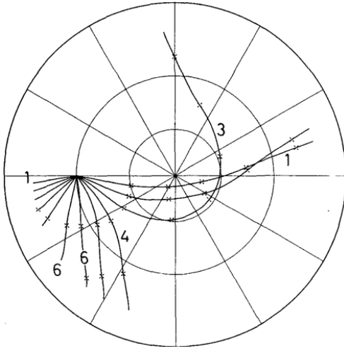
Fig. 16.17 The rays emanating from a point source at 30° N and 180° (nine o'clock), calculated using the observed value of the wind at 300 mb. 17 The crosses mark every 180° of phase, and mark the positions of successive positive and negative extrema. The numbers indicate the zonal wave-number of the ray. The ray paths may be compared with the full linear calculation shown in Fig. 16.18.
