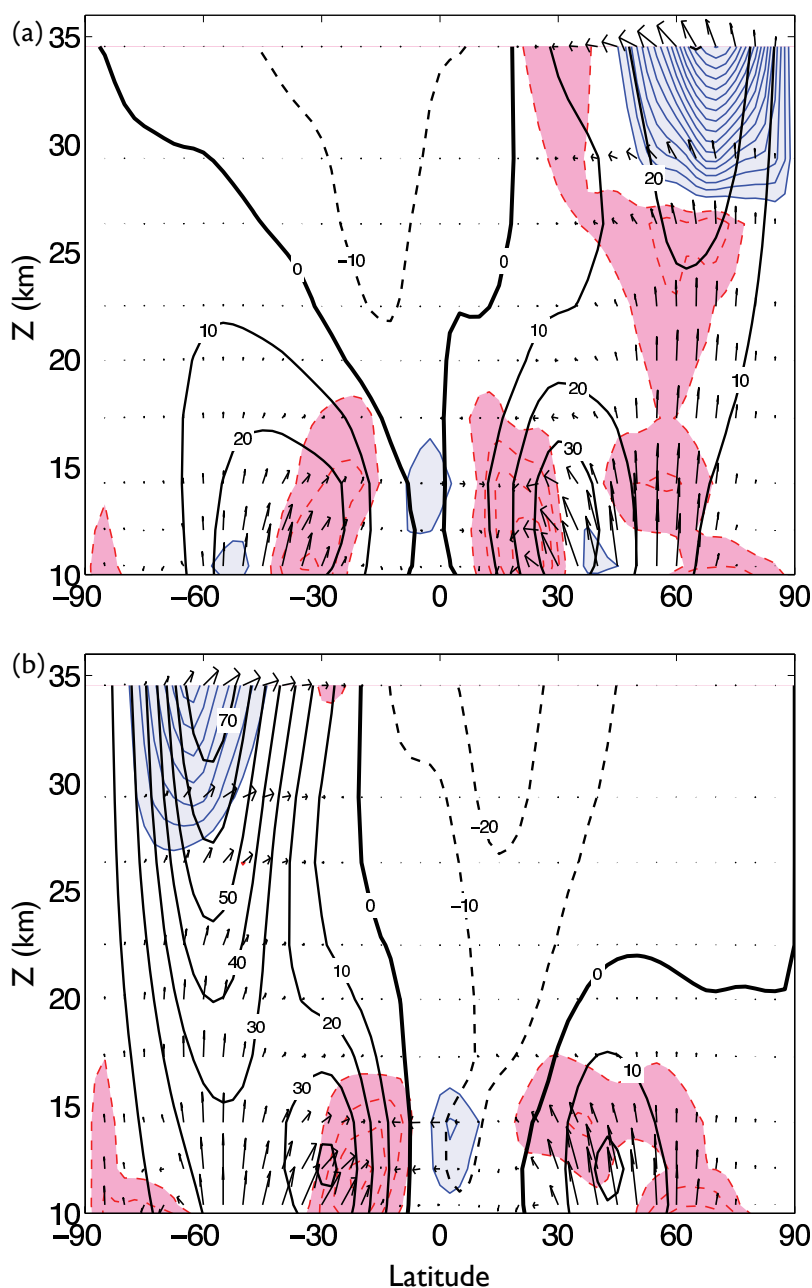
Fig. 17.11 The EP flux vectors (arrows), the EP flux divergence (shaded and light contours) and the zonally averaged zonal wind (heavy contours) for (a) northern hemisphere winter; (b) southern hemisphere winter. Note the almost zero EP values in the summer hemispheres, and strong convergence at high latitudes in the winter hemispheres, leading to poleward residual flow and/or zonal flow acceleration. The EP divergence is shaded for values greater than +1 \text{ m s}^{-1}/\text{day} (light solid contours) and for values less than -1 \text{ m s}^{-1}/\text{day} (light dashed contours). The vertical coordinate is log pressure, extending between about 260 and 10 mb.
