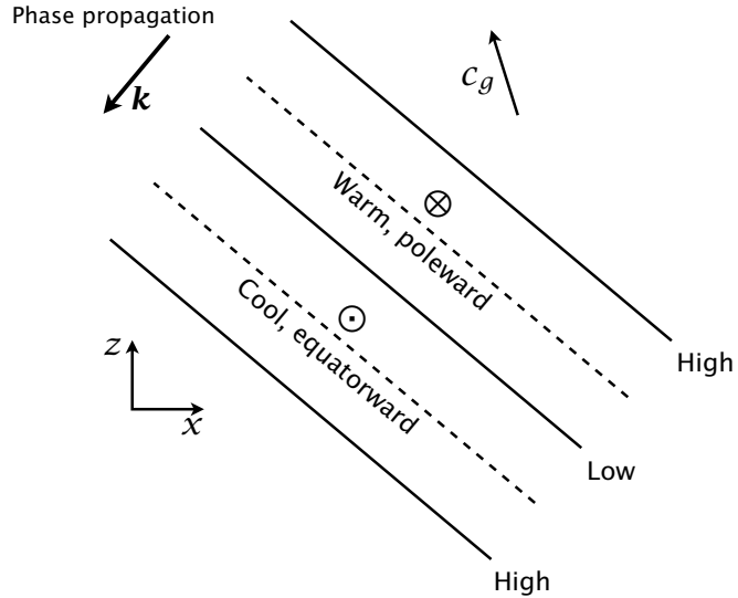
Fig. 16.5 A schematic east-west section of an upwardly propagating Rossby wave. The slanting lines are lines of constant phase and 'high' and 'low' refer to the pressure or streamfunction values. Both k and m are negative so the phase lines are oriented up and to the west. The phase propagates westward and downward, but the group velocity is upward.
