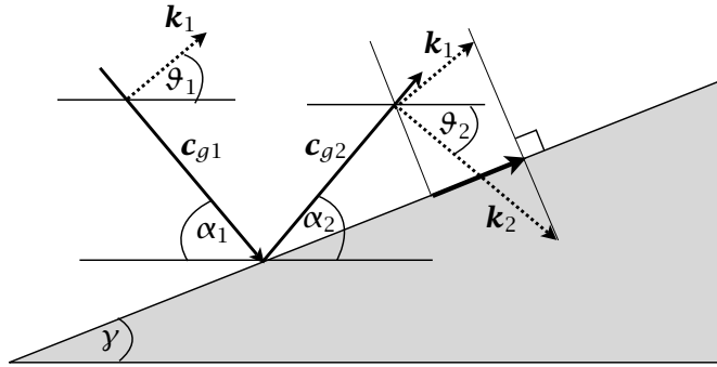
Fig. 7.8 Internal wave reflection from a shallow sloping boundary. The incoming wave vector, k_1 , makes an angle \vartheta_1 with the horizontal, and the incoming group velocity, c_{g1} , makes an angle \alpha_1 = \pi/2 - \vartheta_1 . The group velocity of the reflected wave, c_{g2} , is directed away from the slope, and to satisfy the frequency condition we have \alpha_2 = \alpha_1 . The projection along the slope of the reflected wave vector, k_2 , must be equal to that of the incoming wave vector (the projection is the short thick arrow along the slope), and so the magnitude of the reflected wave vector is larger than that incoming wave.
