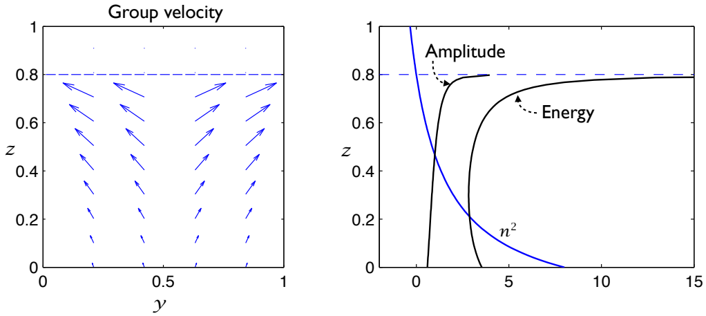
Fig. 16.8 Left panel: group velocity vectors calculated using (16.7) for the parameters shown in Fig. 16.7a, assuming a source at y = 0.5 . Right: profiles of n^2 , wave amplitude and energy. The horizontal line at z = 0.8 marks a turning surface, and the group velocity turns away from it.
