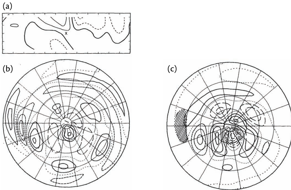
Fig. 16.14 Numerical solution of a baroclinic primitive equation model with a deep heat source at 15° N and a zonal flow similar to that of northern hemisphere winter. (a) Height field in a longitude height at 18° N (vertical tick marks at 100, 300, 500, 700 and 900 mb); (b) 300 mb vorticity field; (c) 300 mb height field. The cross in (a) and the hatched region in (c) indicate the location of the heating. 8
