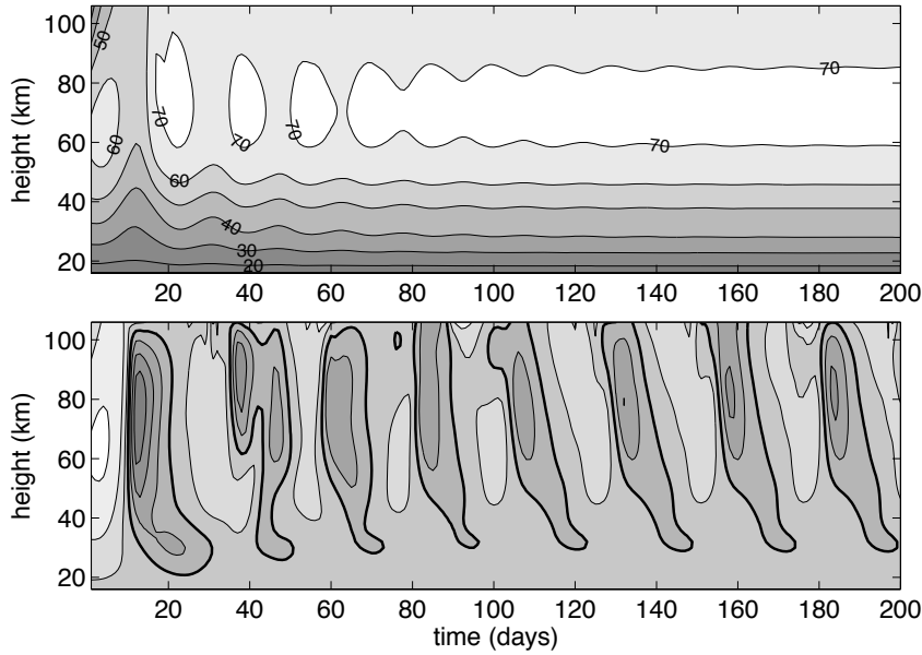
Fig. 17.27 Evolution of the zonal mean zonal wind in a case with steady wave forcing with a value of 200 in the top panel and 300 in the lower panel. In the bottom panel the contours are every 20 \text{ m s}^{-1} , positive values have lighter shades and the zero contour is heavy.
