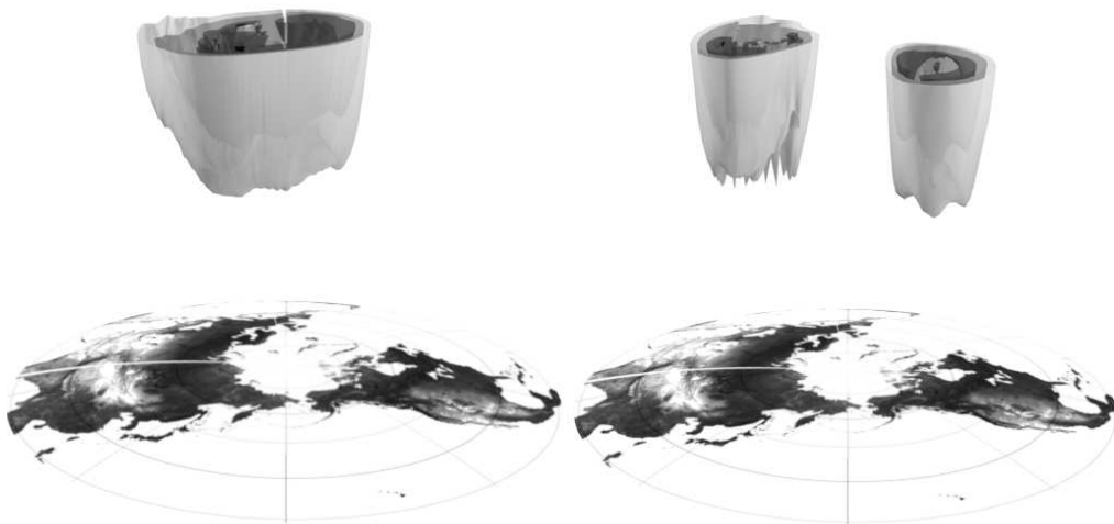
Fig. 17.6 The edge of the stratospheric polar vortex in 1984. Plotted is the 35 PVU isosurface of Q^* = Q(\theta/\theta_0)^{4.1} , where Q is Ertel PV and \theta_0 = 475 K. The vertical coordinate is potential temperature. Like Q , Q^* is materially conserved in adiabatic flow. It is approximately constant at the vortex edge, roughly compensating for the change in density with height that affects the Ertel PV. The left panel shows the vortex in a fairly usual state, and the right panel shows a split vortex following a stratospheric sudden warming. 11
