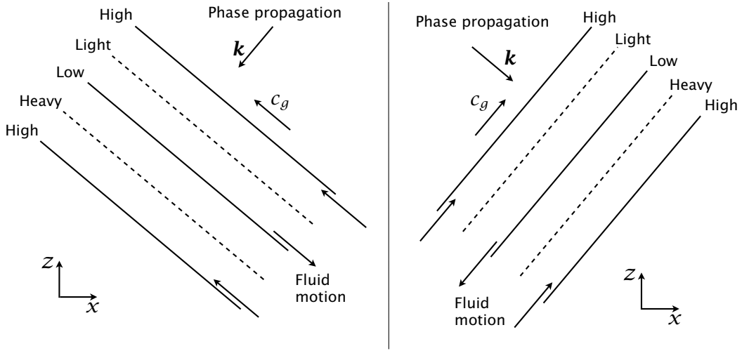
Fig. 17.9 Phase relationships for two examples of upwardly propagating gravity waves. The sketch on the left shows waves propagating to the left, with k < 0 , and the one on the right sketch shows waves with k > 0 . Lines of constant phase are solid and dotted lines, with 'high' and 'low' referring to pressure and 'light' and 'heavy' referring to density and corresponding to warm and cold, respectively. In both sketches m is negative and the group velocity is directed upwards and phase propagates downwards. For hydrostatic flow the phase lines would be nearly horizontal. The figure may be compared with Fig. 7.4.
