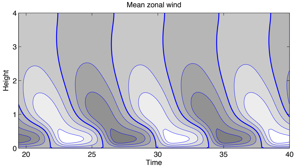
Fig. 17.20 Time height section of nondimensional zonal wind in a numerical solution of (17.68), showing the last 20 time units of the same integration as Fig. 17.19. Contours are plotted every 0.2 units, positive winds are shaded darker and the zero contour is thicker.
