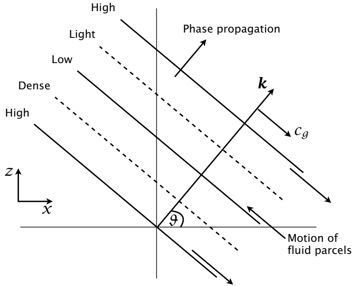
Fig. 7.4 An internal wave propagating in the direction k . If the motion is in the x - z plane then both k and m are positive for the wave shown. The solid lines show crests and troughs of constant pressure, and the dashed lines the corresponding crests and troughs of buoyancy (or density). The motion of the fluid parcels is along the lines of constant phase, as shown, and is parallel to the group velocity and perpendicular to the phase speed.
