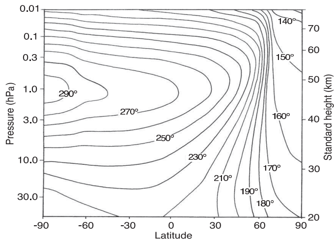
Fig. 17.1 The zonally averaged radiative-equilibrium temperature in January; that is, the temperature that would arise in the absence of fluid motion in the stratosphere. 3
