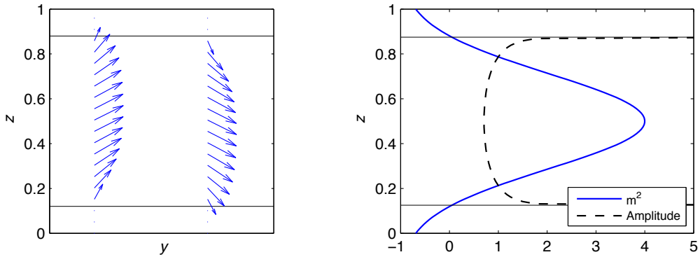
Fig. 7.15 Left panel: Group velocity vectors for upward and downward propagating gravity waves in a stratification illustrated in Fig. 7.14, calculated using (7.122). Right panel: The values of m^2 and the amplitude of the wave, the latter varying as m^{-1/2} . The thin horizontal lines in both panels indicate the height at which m^2 = 0 .
