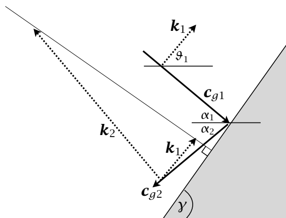
Fig. 7.9 As for Fig. 7.8, but now showing reflection from a steep slope. The wave is back-reflected down the slope, and in this example the magnitude of the reflected wave is again larger than that of the incoming wave.
