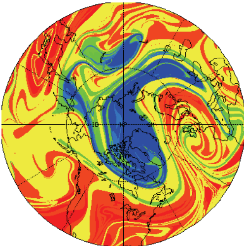
Fig. 17.4 The tracer distribution in the northern hemisphere lower stratosphere on 28 January 1992. The tracer was initialized on 16 January 1992 by setting it equal to the potential vorticity field calculated from an observational analysis, and then advected for 12 days by the observed wind fields. 7
