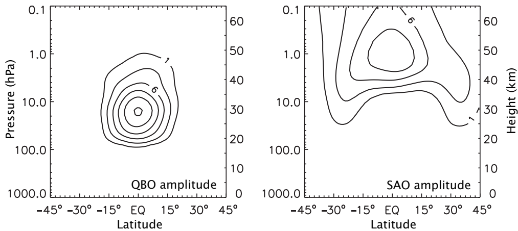
Fig. 17.15 The amplitudes (essentially the root-mean square of the zonally-averaged wind of the oscillations after temporal filtering, with contours at 1, 3, 6, 9, 12 and 15 \text{m s}^{-1} ) of the QBO and the SAO. The QBO evidently extends roughly from 15° S to 15° N and from 100 hPa to 1 hPa (18 km to 50 km). The SAO is broader, higher, weaker and faster. 26
