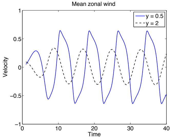
Fig. 17.19 The evolution of the mean zonal wind at two different levels in a numerical solution of (17.68). All the variables are nondimensional, with the only parameter in the problem being viscosity, and here \hat{\nu} = 0.15 . A small perturbation is added to \hat{u} , and relatively quickly the solution becomes periodic.
