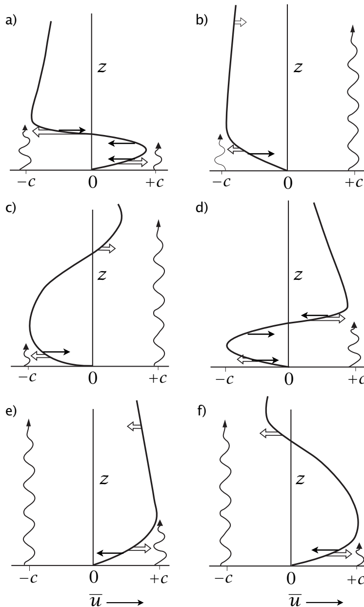
Fig. 17.18 Schema of the evolution of the QBO with gravity-wave forcing from below, following an initial perturbation illustrated in Fig. 17.17. 32 The solid lines show the mean flow and the wavy lines indicate the propagation of gravity waves. Horizontal double arrows indicate wave forcing and single arrows indicate viscous relaxation. The panels are at successive times, with the top four panels showing a half cycle, and panels (d), (e) and (f) are mirror images of (a), (b) and (c). Wave-induced acceleration of the mean flow occurs preferentially near critical levels where \bar{u} = c .
