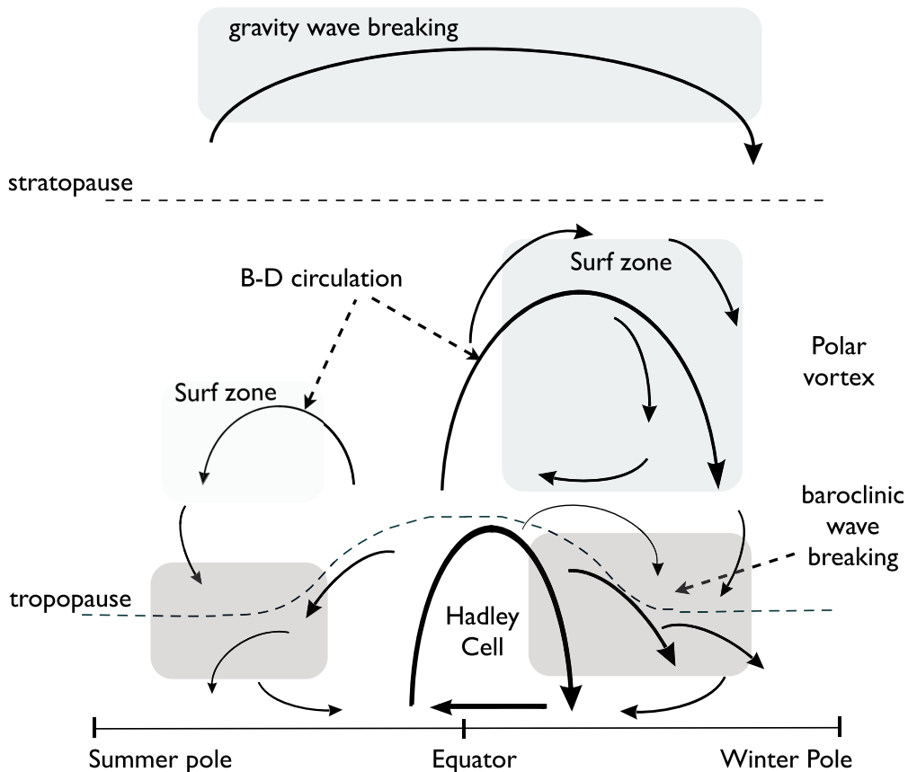
Fig. 17.8 A schema of the residual mean meridional circulation of the atmosphere. The solid arrows indicate the residual circulation (B-D for Brewer–Dobson) and the shaded areas the main regions of wave breaking (i.e., enstrophy dissipation) associated with the circulation. In the surf zone the breaking is mainly that of planetary Rossby waves, and in the troposphere and lower stratosphere the breaking is that of baroclinic eddies. The surf zone and residual flow are much weaker in the summer hemisphere. Only in the Hadley Cell is the residual circulation comprised mainly of the Eulerian mean; elsewhere the eddy component dominates.
