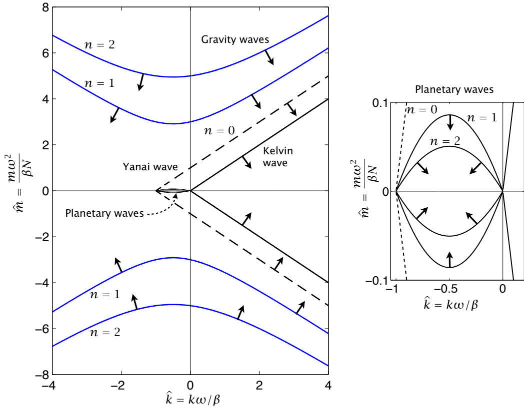
Fig. 17.10 The dispersion relation plotted in \hat{m} - \hat{k} space, using (17.15). Shown are gravity waves, the Yanai wave and the Kelvin wave for positive and negative \hat{m} , with the plot at the right showing a magnification of the region near the origin. The arrows in the figure indicate the group velocity, which, being the gradient of the frequency, is perpendicular to the curves. Upward propagating waves occur for negative m . Compare with Fig. 8.2.
