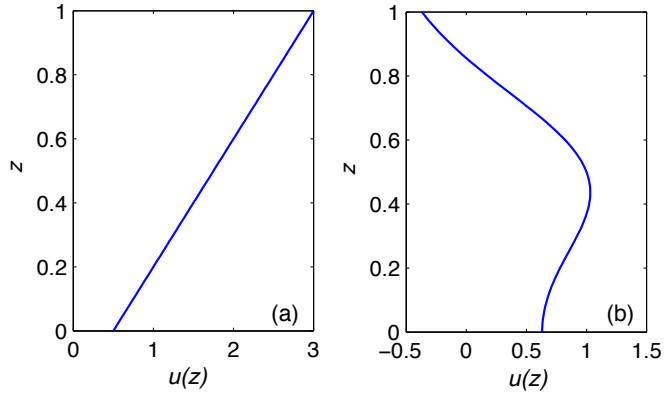
Fig. 16.7 Two profiles of non-dimensional zonal wind used in the calculations illustrated in Fig. 16.8 and Fig. 16.9. (a) is a uniform shear that gives rise to a turning latitude, and (b) shows a profile in which the zonal wind diminishes to zero aloft, giving rise to a critical layer.
