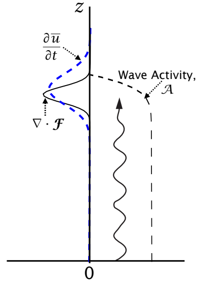
Fig. 17.24 Schematic of a model of a stratospheric warming. Upward propagating Rossby waves (wavy line) reach the stratosphere and break, and the wave activity (dashed line) diminishes. In the breaking region the EP flux divergence is negative ( \nabla \cdot \mathcal{F} < 0 ), inducing a westward acceleration ( \partial \bar{u} / \partial t < 0 ) over a somewhat broader region. See also Fig. 17.25.
