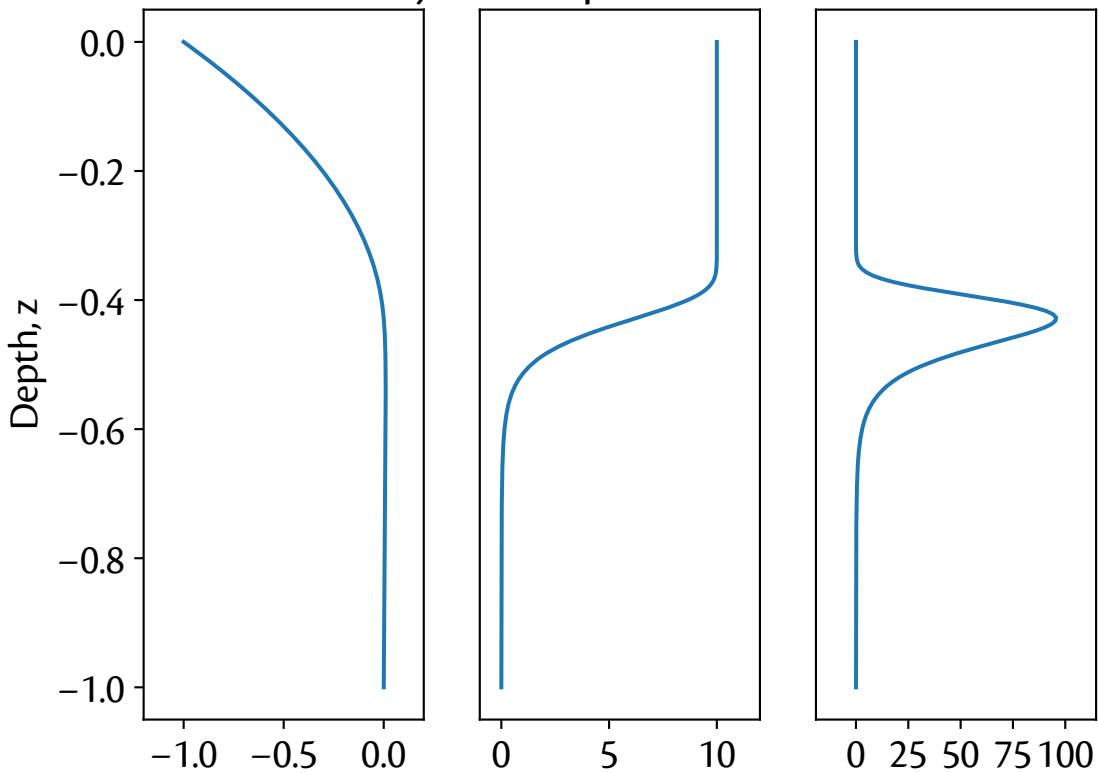
Vertical velocity
