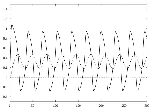
Time-series of typical solution.
