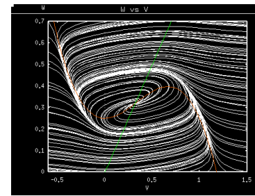
Phase plane of typical solution with flow added.
