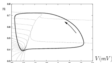
Isochrons for a Hodgkin-Huxley neuron http://www.scholarpedia.org/article/Isochron
