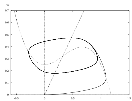
Phase plane of typical solution.
