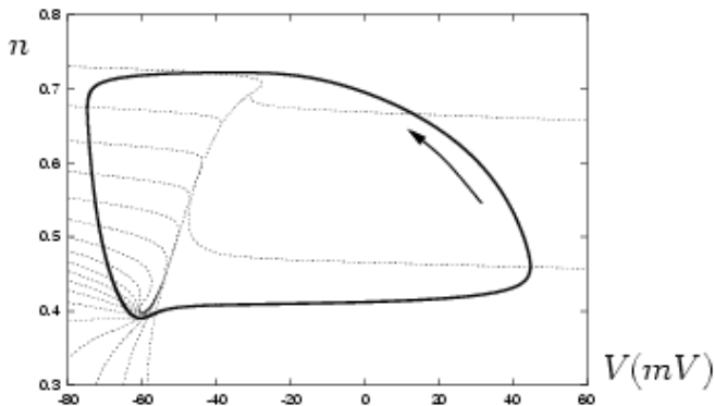
Isocrons for a Hodgkin-Huxley neuron ( http://www.scholarpedia.org/article/Isochron )
