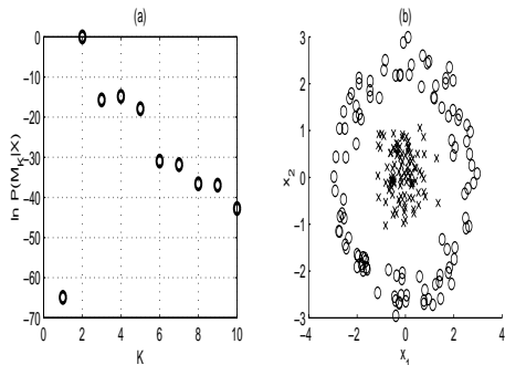
Figure 3: Ring data set: (a) \ln P(M_K | X) & (b) resultant partitioning. For this example there are no errors.
