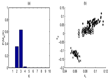
Figure 5: Iris data set: (a) P(M_K | X) & (b) resultant partitioning. For this example there are three errors, corresponding to an accuracy of 98%.
