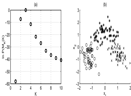
Figure 6: Wine recognition data set: (a) \ln P(M_K | X) & (b) resultant partitioning. For this example there are four errors, corresponding to an accuracy of 97.75%.
