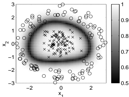
Figure 4: Ring data set: Maximum partition posterior.
