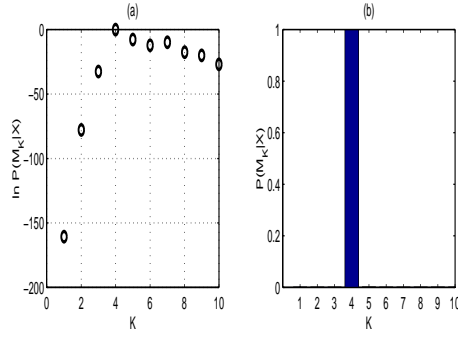
Figure 1: Simple data set: (a) \ln p(M_K | X) and (b) p(M_K | X) . Note the clear maxima at K = 4 .
