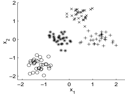
Figure 2: Simple data set: Data partitioning in the transformed space. For this simple example there are no errors.
