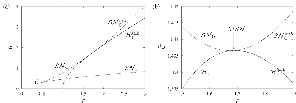
Figure 15. (a) Part of the bifurcation diagram of fixed points of \mathcal{P}_{F,G,0} , for \epsilon = 0.01 . (b) Magnification of (a) of box M around the point \mathcal{H}\mathcal{S}\mathcal{N} . The latter graph has been deformed by an affinity, plotting couples (F, \tilde{G}) , where \tilde{G} = G - 1.5 \times (F - 1.5) .
